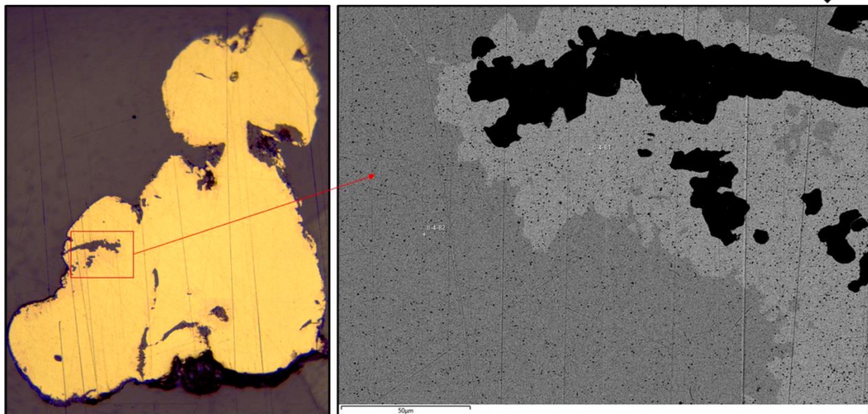
Image: Polished section and SEM image of grain II-4 from sample SB-10
